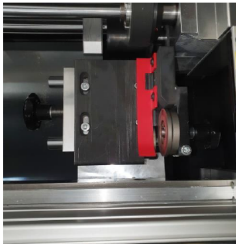
Longitudinal cutting device (additional Cutting of the sheets possible)
