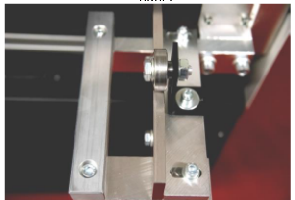
Guide on the sheet metal outlet
