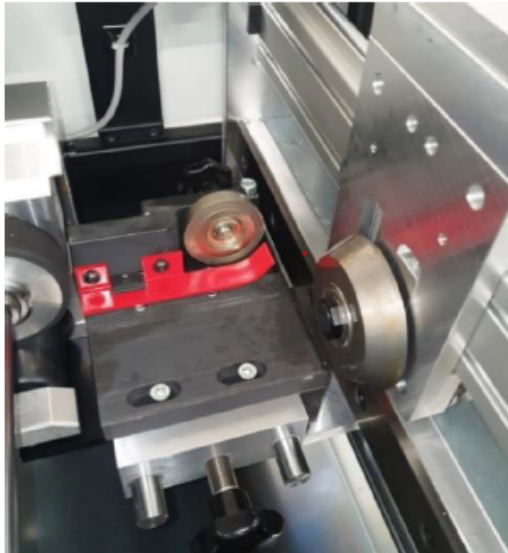
Slitting and cut-to-length knives
